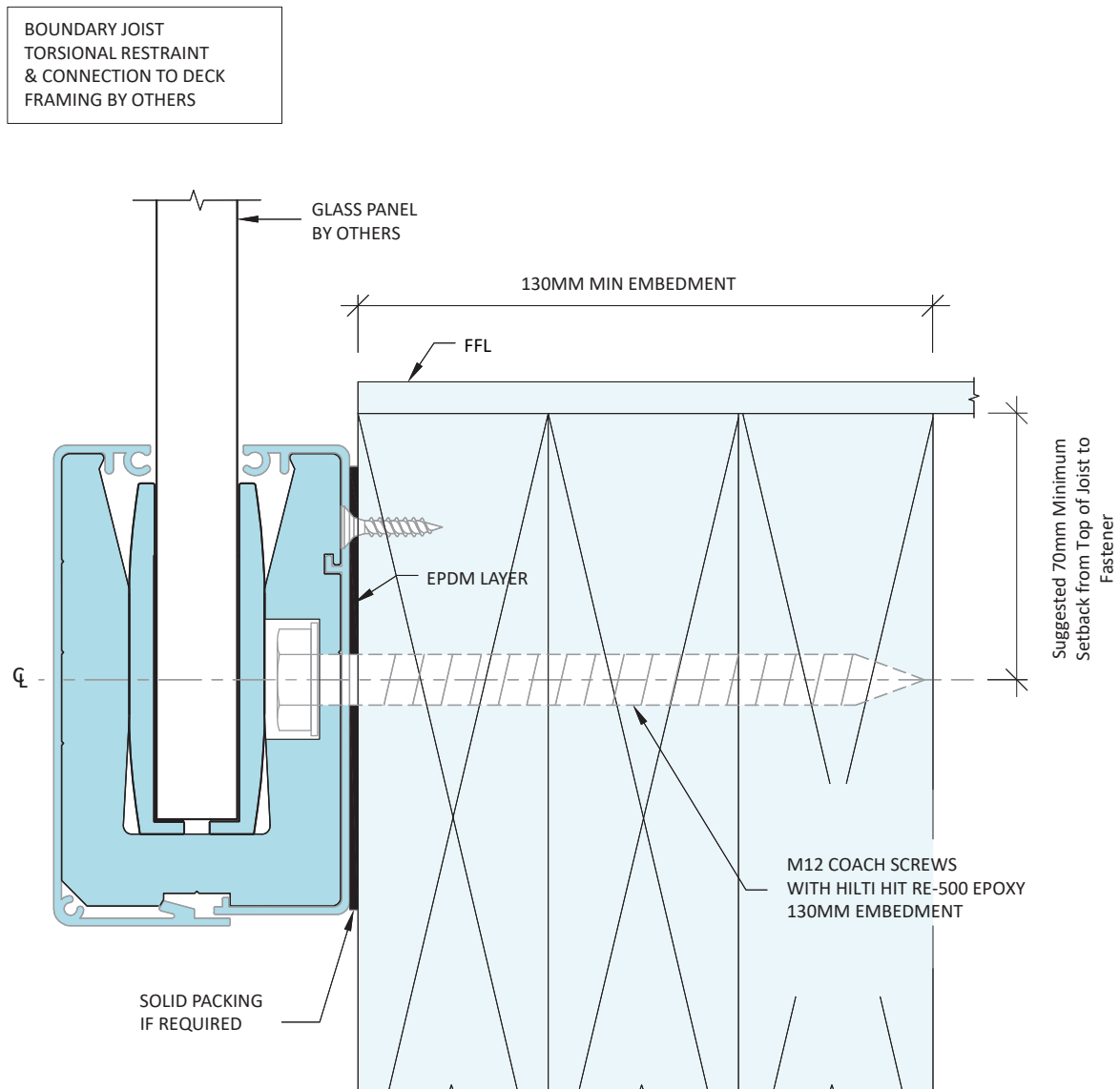
3B CONNECTION TYPE 3B - TIMBER DECK WITH COACH SCREWS SCALE 1:2
