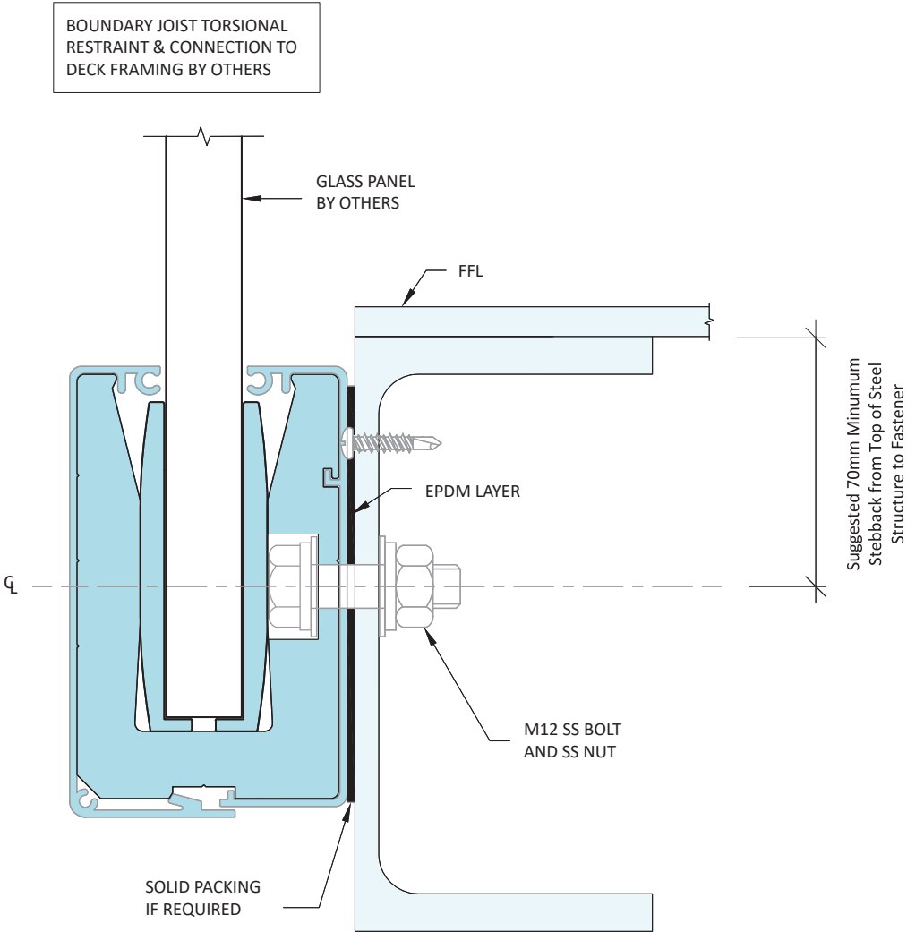
1 CONNECTION TYPE 1 - STEEL DECK SCALE 1:2
